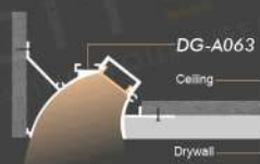
Recessed Corner Trimless Profile For Cove Lighting Wallwasher
