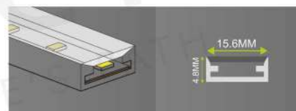
DG-LF-T09 (CLEAR) (15.6 X 4.8)
