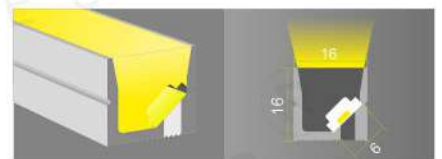
DG-24V-3D-01-3K 3D BENDING (16x16)
